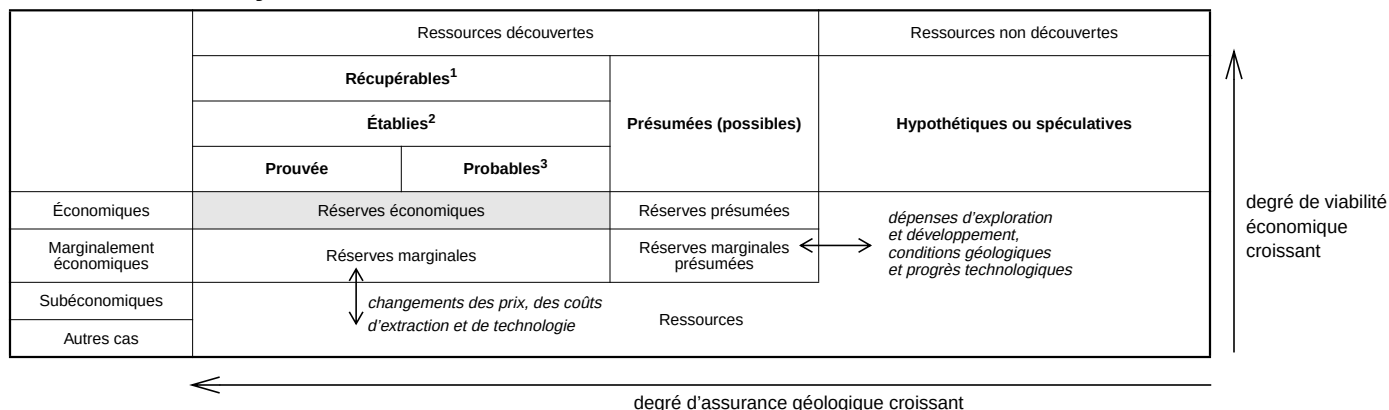
Figure 3.1 Carré de McKelvey
